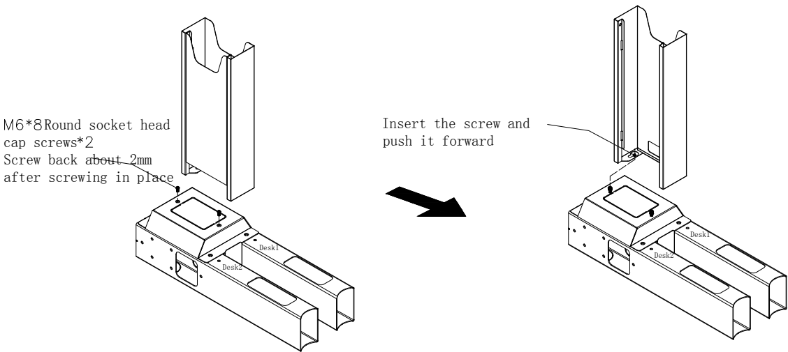
Assemble the optional cable box on the table
