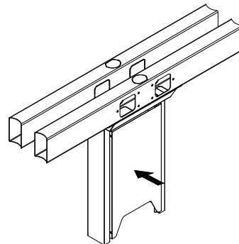
04 Assemble the cover for the cable column
