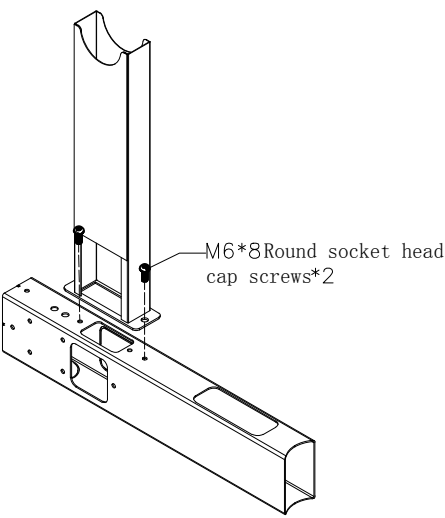
Assemble the optional cable column
