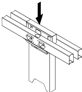
05 Snap the cover
