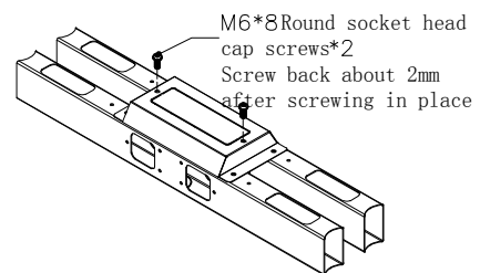
04 Assemble the cover for the cable column
