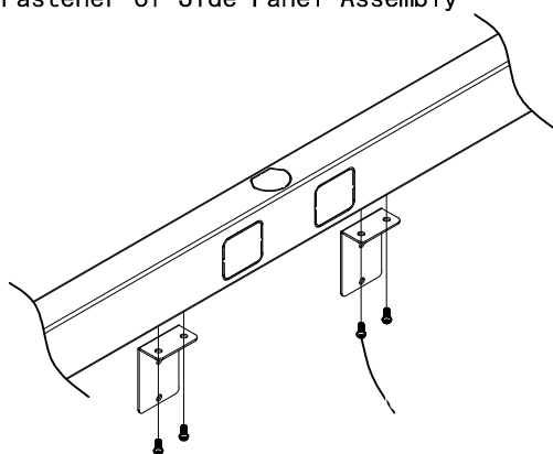
03 Assemble the Side panel connector (panel inside)
