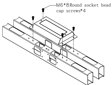
03 Assemble the Cable Column
