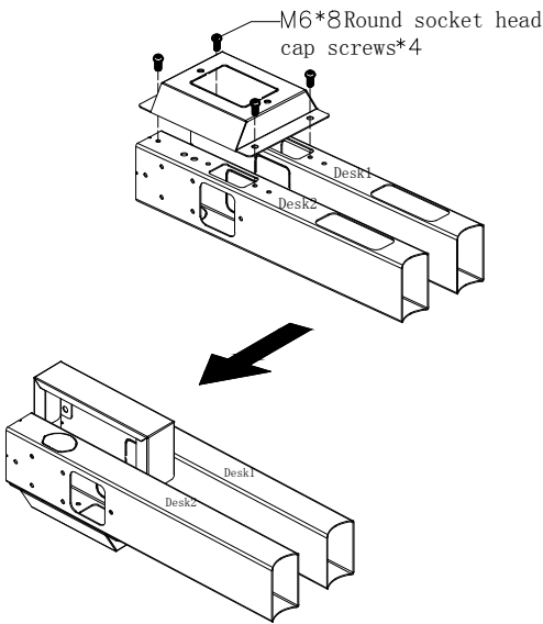
Assemble the optional desk Connector
