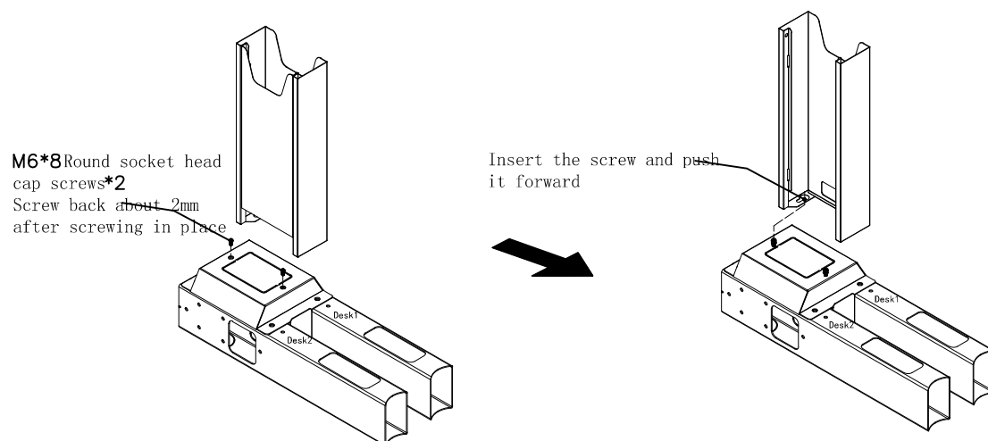
Bottom View
